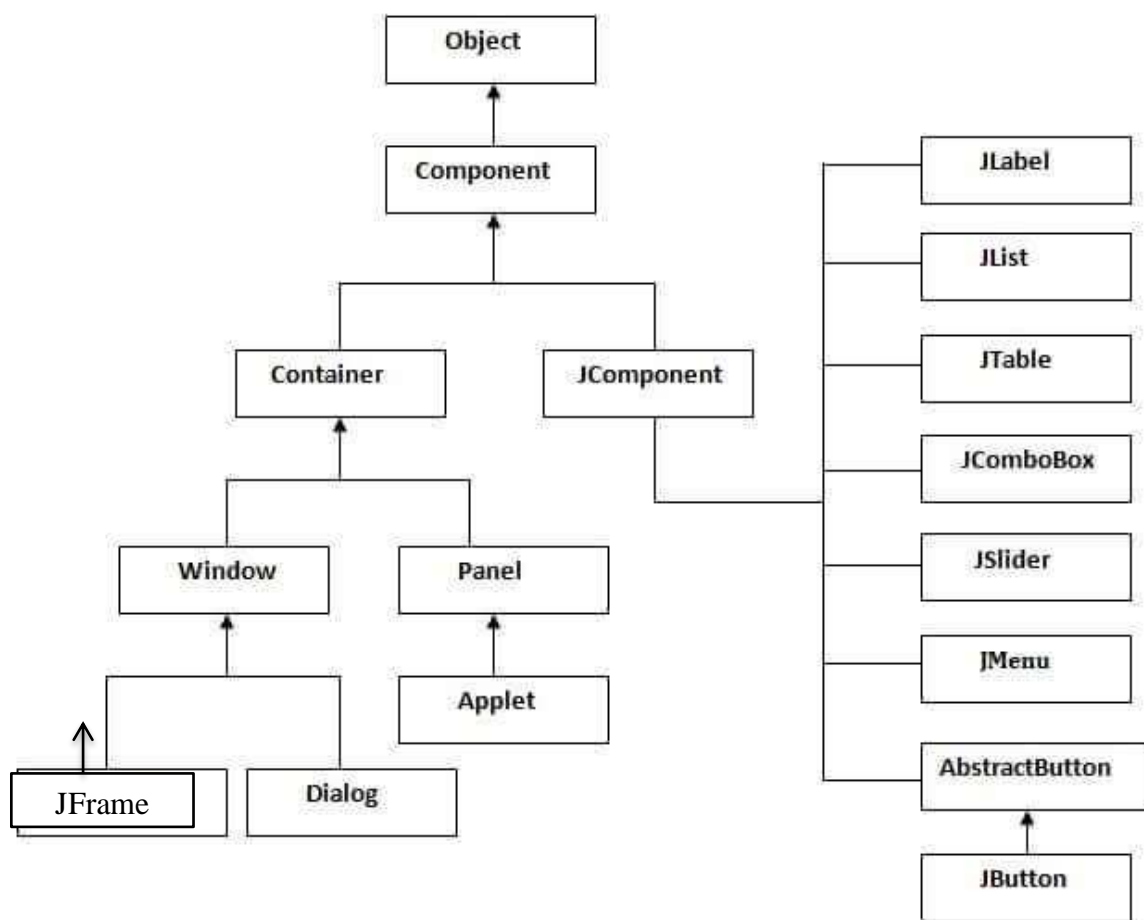
Figure 1: Swing Hierarchy
